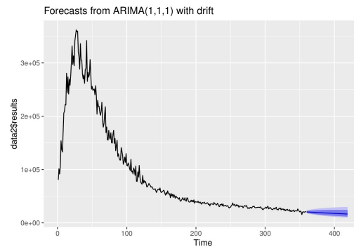
Figure 8: Prediction results
