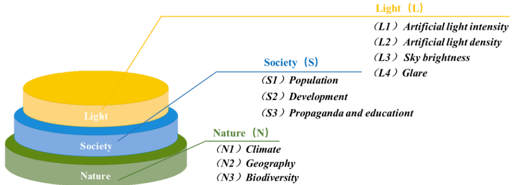
Figure 3: Hierarchy diagram
