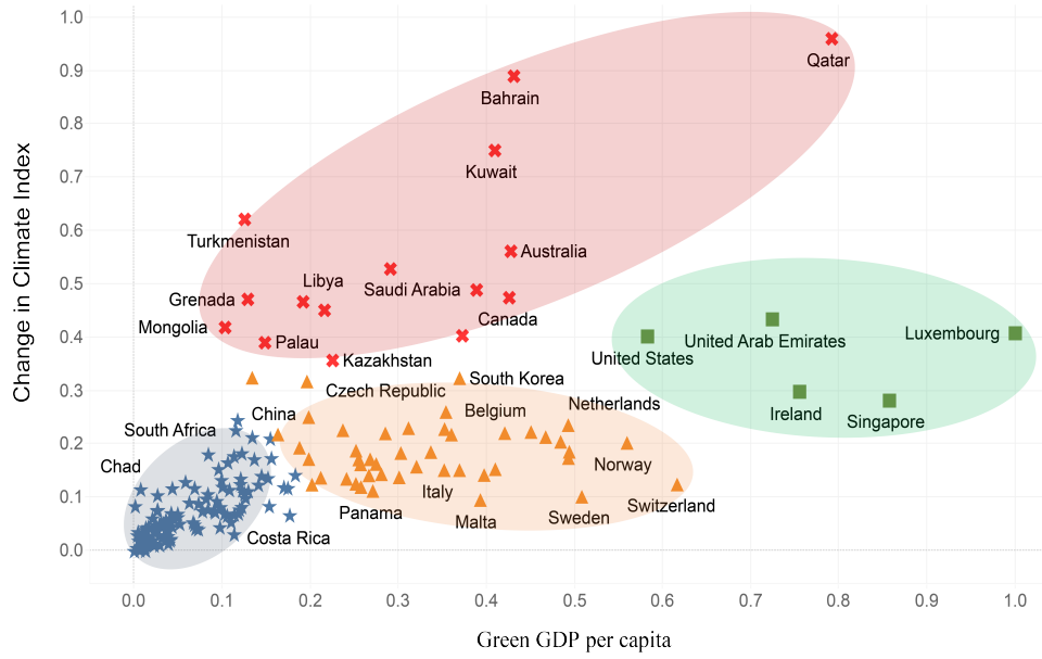
Figure 8: Kmeans-results
